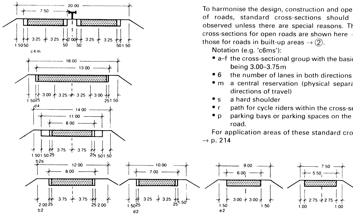
① Standard cross-sections for open roads
